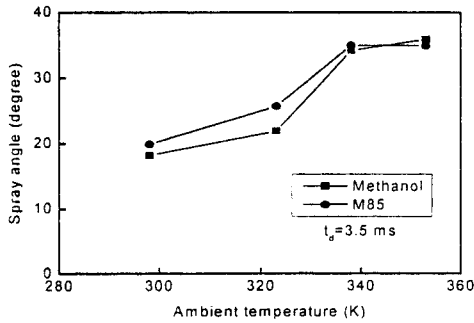
Fig. 7 Comparison of spray angles between methanol and M85 for ambient temperature
