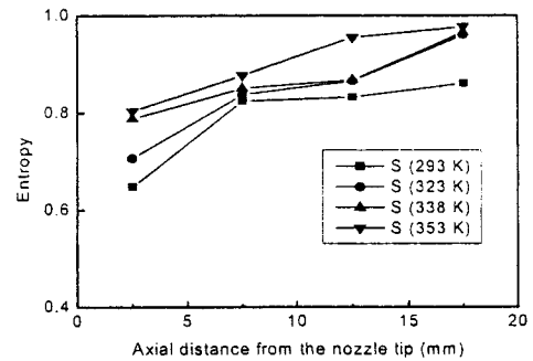
Fig. 9 Entropy variation for M85
