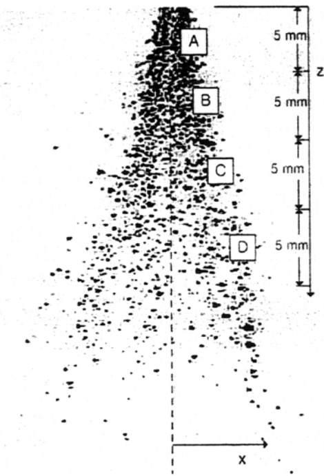
Fig. 3 Typical spray image for analysis
