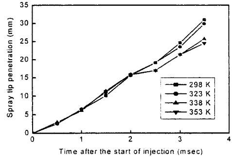
Fig. 5 Spray tip penetrations for the lapse of time and ambient temperature
