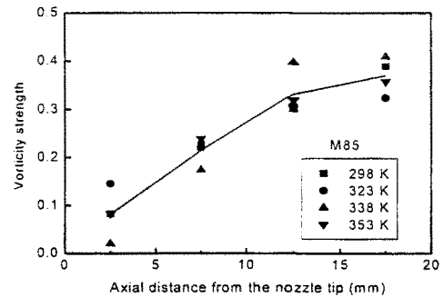
Fig. 12 Variation of vorticity strength for distance from the nozzle tip
