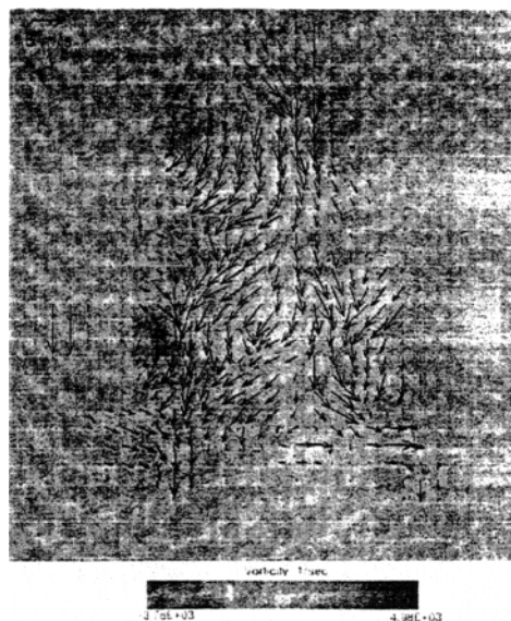
Fig. 10 An example of PIV image interrogated on whole spray for methanol at T_{\text{amb}}=323 K
